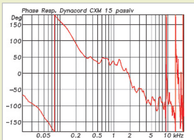
Fig. 2: Phase response of the CXM 15 in passive mode
