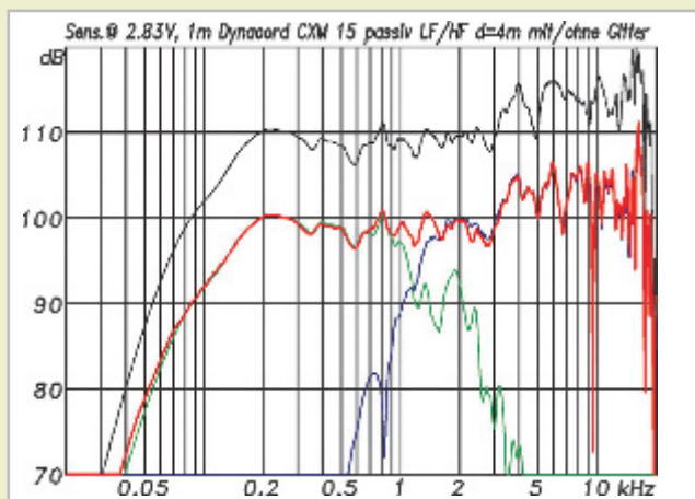
Fig. 1: The frequency response and sensitivity of the CXM 15 (red) as well as the LF (green) and HF paths (blue) with passive crossover. Moved 10 dB upwards and shown in black: the frequency response without the grille
