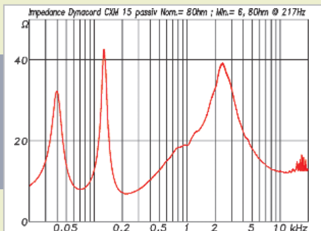
Fig. 4: Impedance curve of the CXM 15 in passive mode showing the minimum impedance of 6.8 ohms at 217 Hz and the tuning frequency of the bass-reflect resonator at 70 Hz
