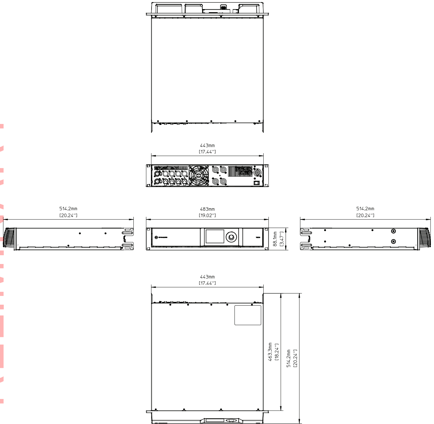
Fig. 2: Dimensions: TGX
