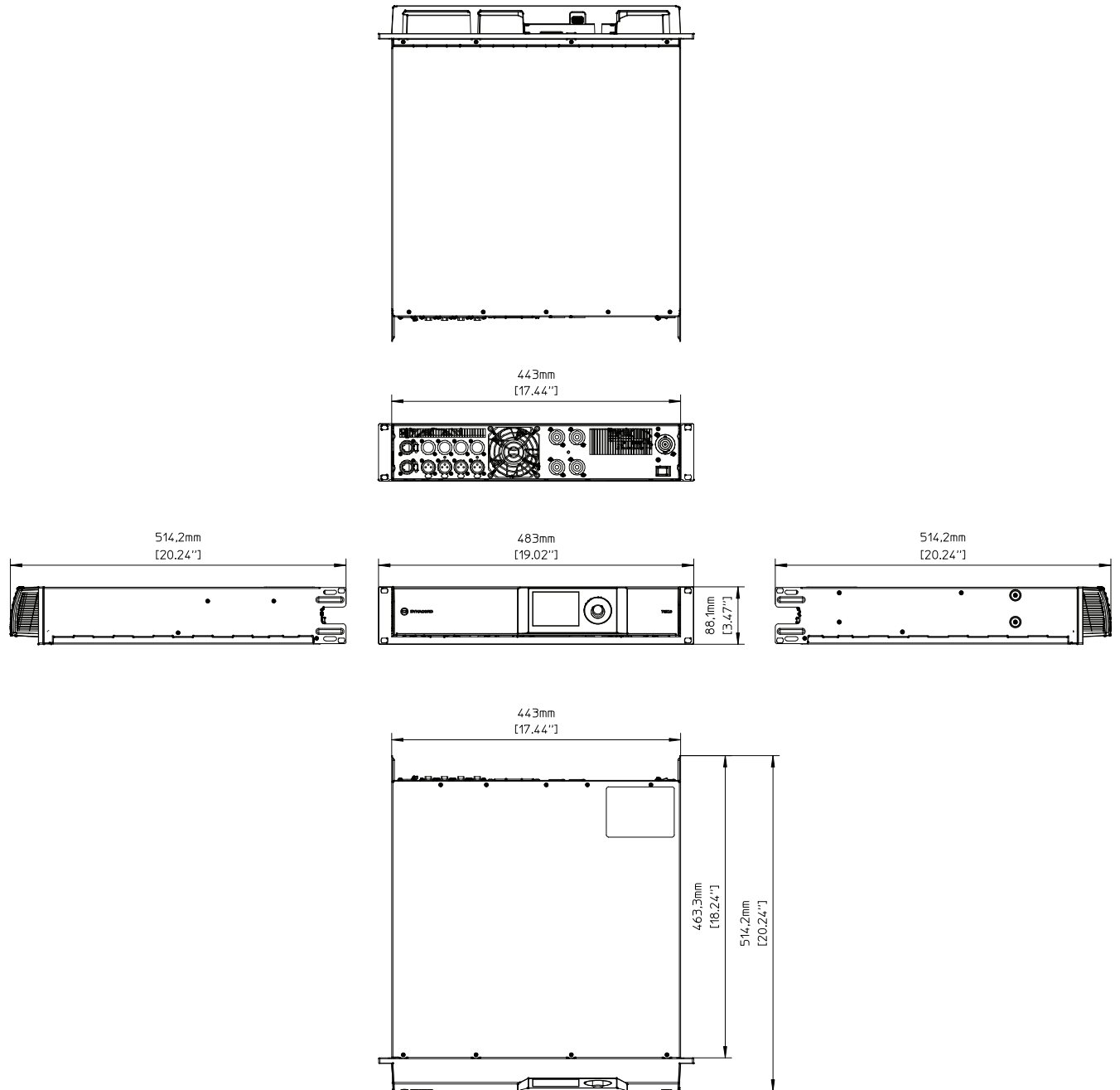
Figure 9.2: Dimensions: TGX
