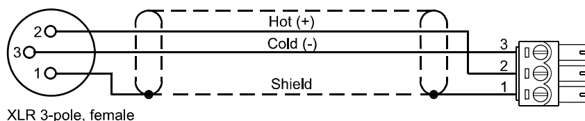
XLR 3-pole, female
