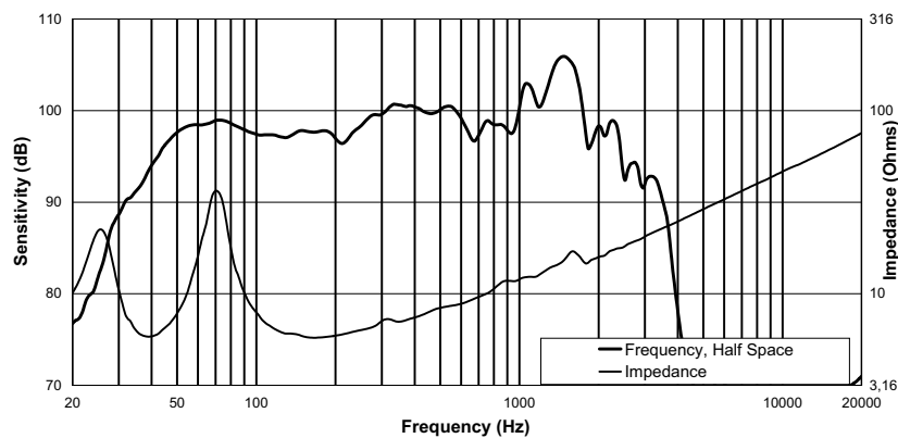
Illustration 2: Frequency Response
