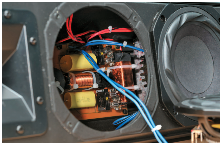
Looking into the interior of the TS400 at the generously dimensioned passive crossover with light bulbs for overload protection. The housing is constructed from an aluminium strand-cast profile
