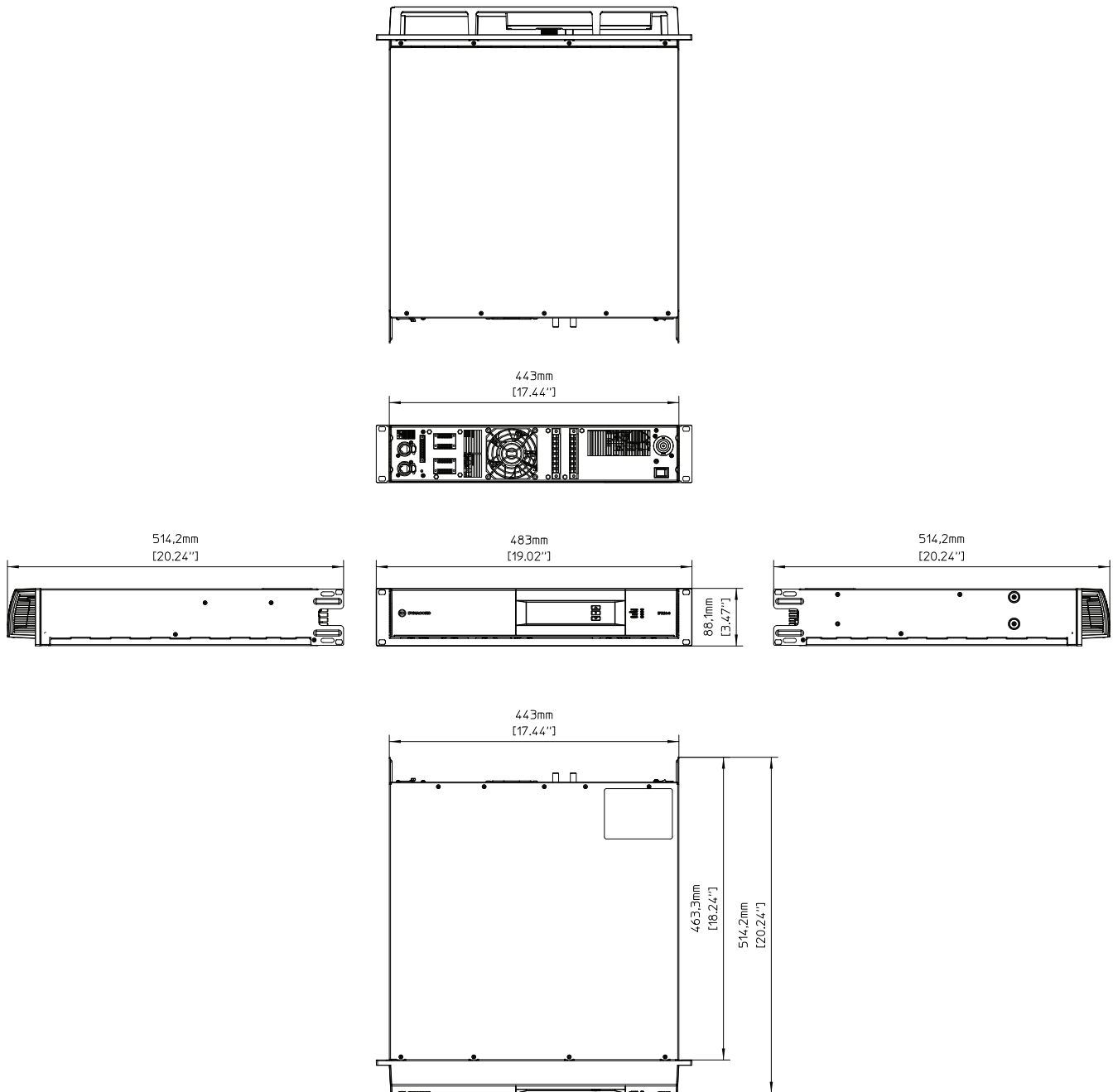
Figure 8.2: Dimensions: IPX
