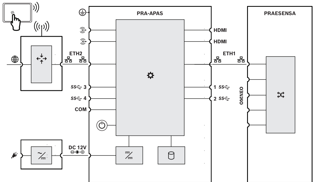
Connection and functional diagram
